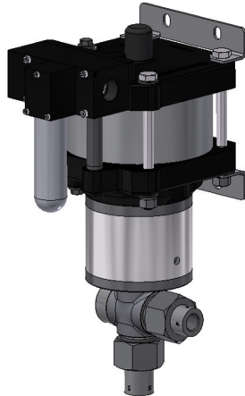
GSF150 (L) single acting, single air drive head with distance piece (Standard = Bottom inlet)
